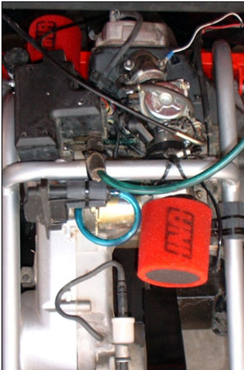
GY6 Engine with Uni Filter
