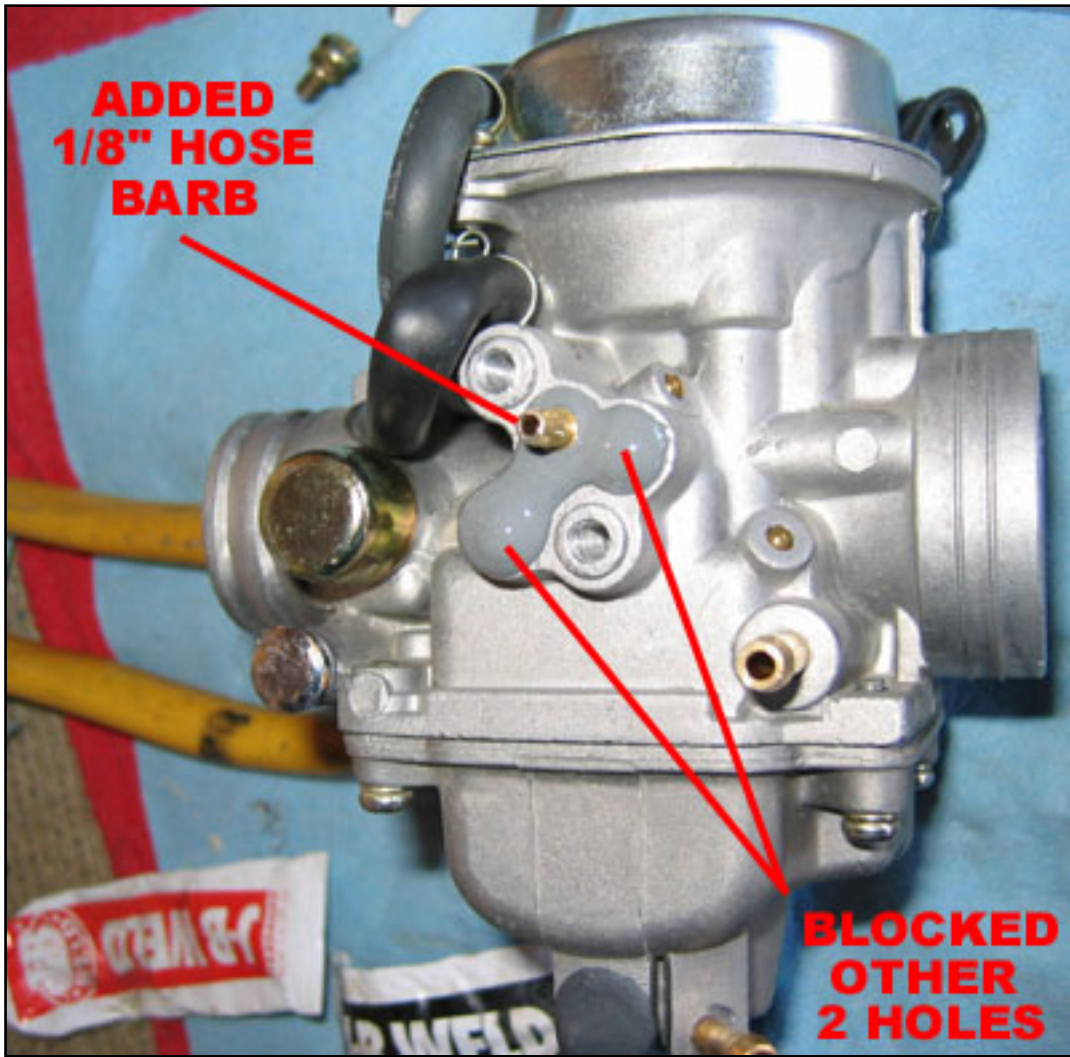
Hose Barb added for Plunger Primer System
